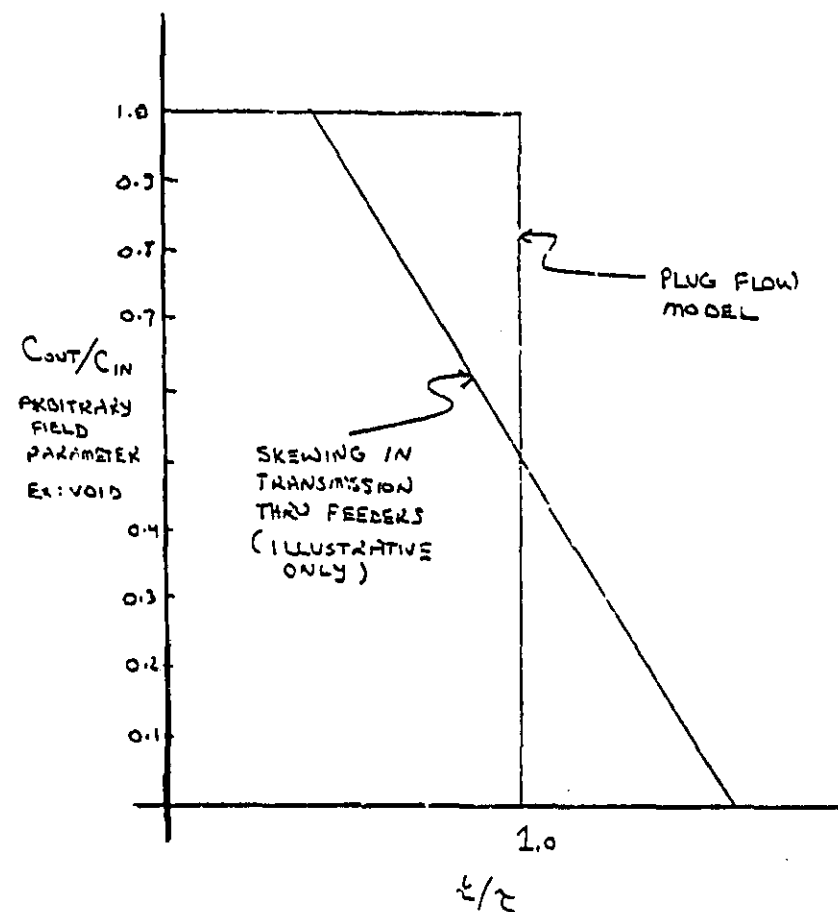
Figure 3.7 Transmission of a step change using the plug flow model and a feeder model with skewing due to differences in transit times.
