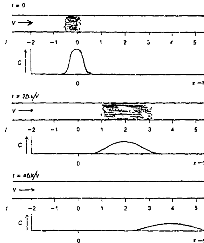
Figure 3.5 Illustration of convection and diffusion.
